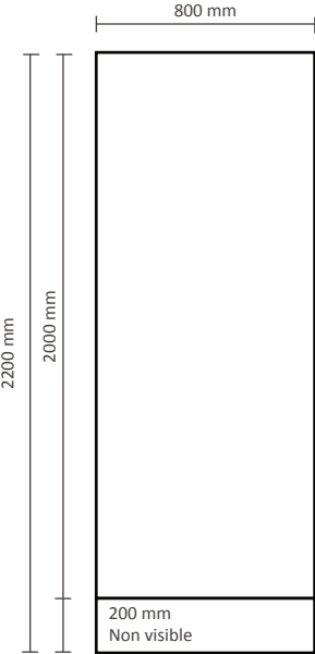
80x200cm RBCUBE080
